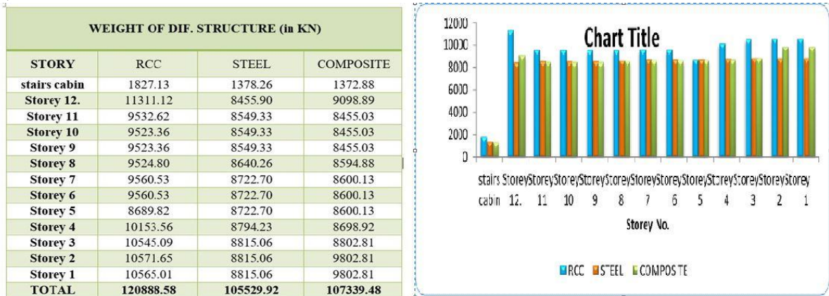
Figure 2. Weight of the structure
