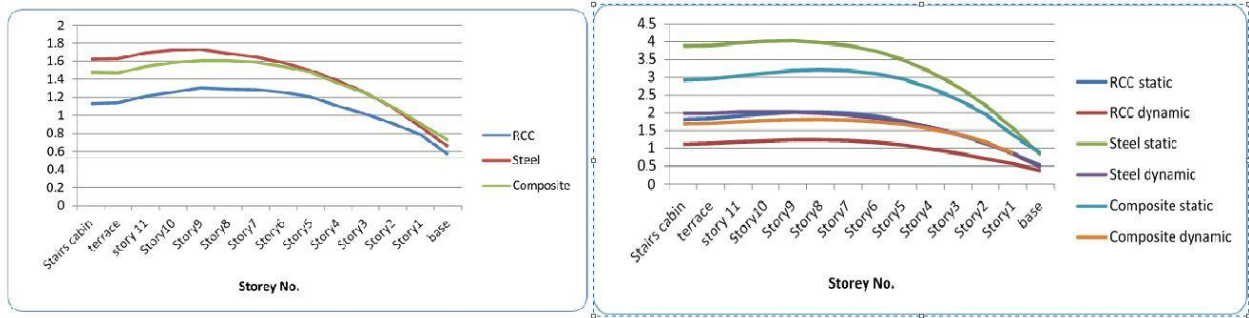
Figure 6. Storey drift for static and dynamic analysis in x-y direction
