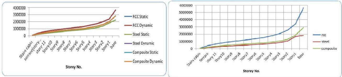
Figure 5. Storey stiffness for static and dynamic analysis in x- y direction
